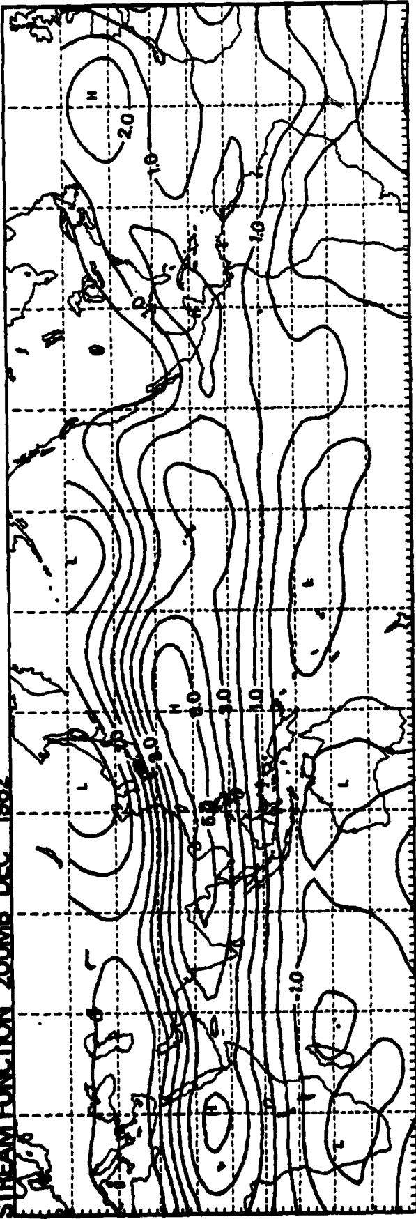
STREAM FUNCTION 200MB DEC 1982
